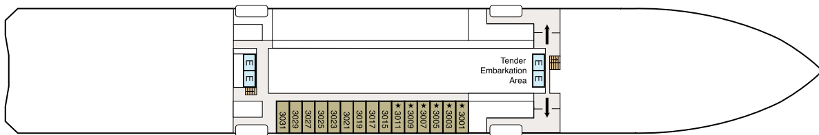
DECK 3
